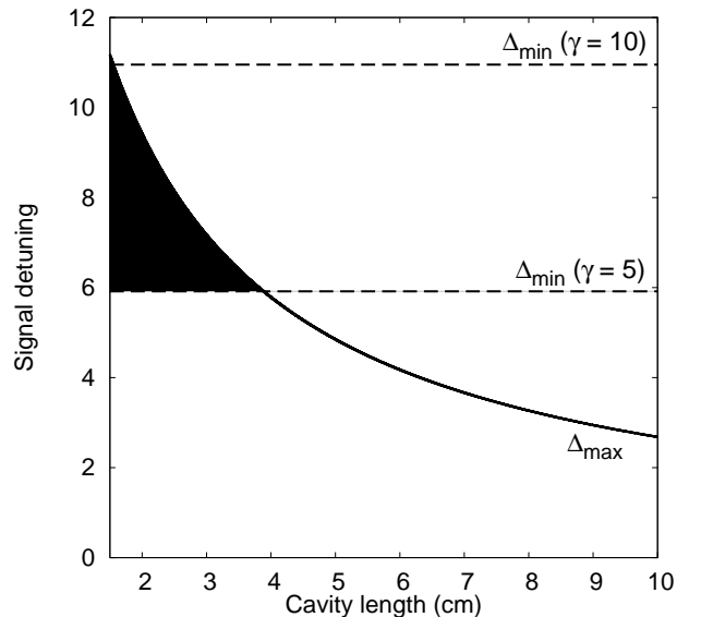
FIG. 2: Solid lines : values of maximal detuning authorized by mode selection when cavity length is varied between 1.5 cm and 10 cm. Dashed lines : minimal detuning permitted by the conditions of the Hopf bifurcation for two different values of \gamma : 5 and 10.
