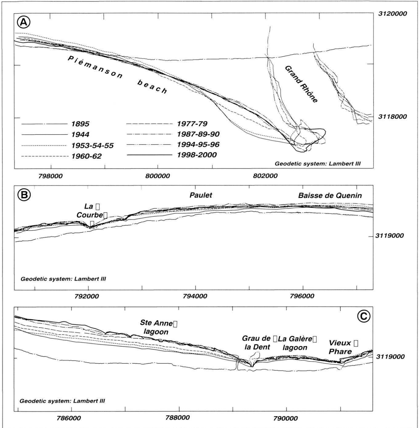
Fig. 7 – Shoreline changes on the littoral of Faraman between 1895 and 2000.
