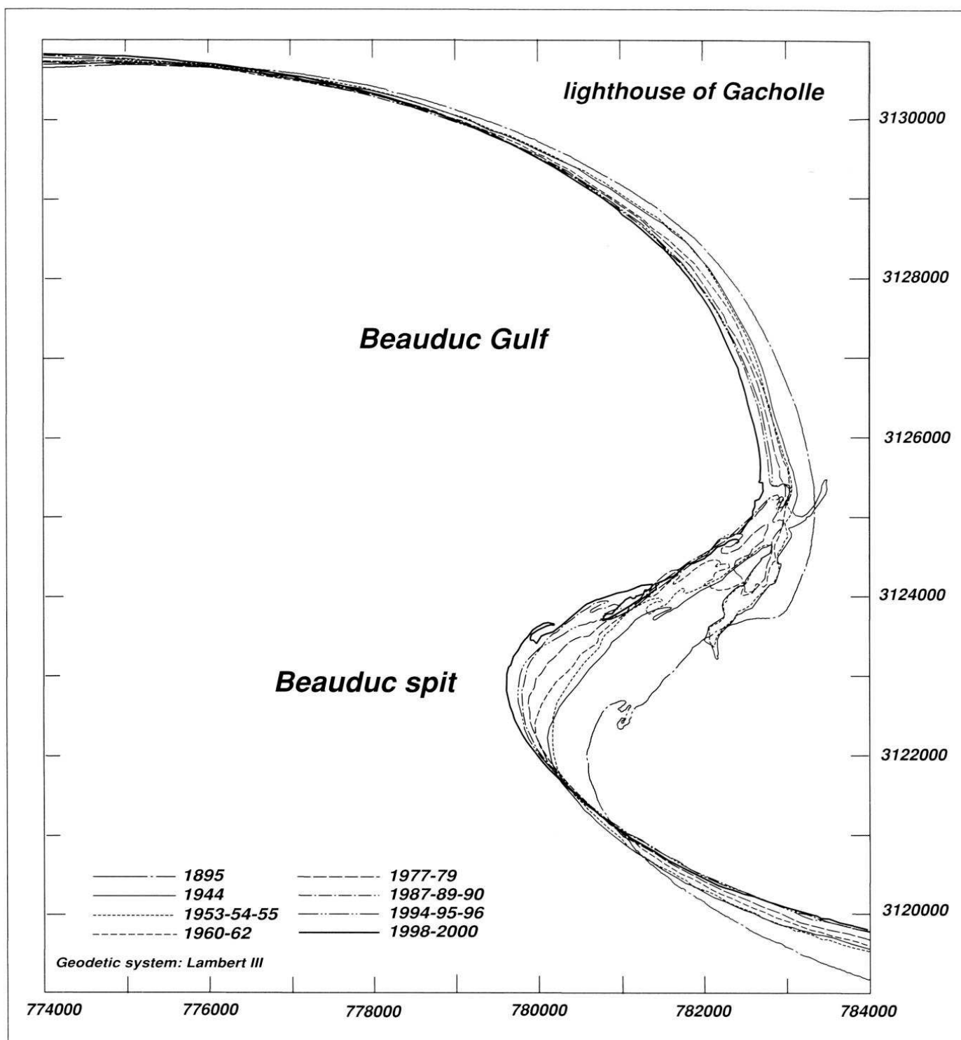
Fig. 8 – Shoreline changes on the spit and gulf of Beauduc between 1895 and 2000.
