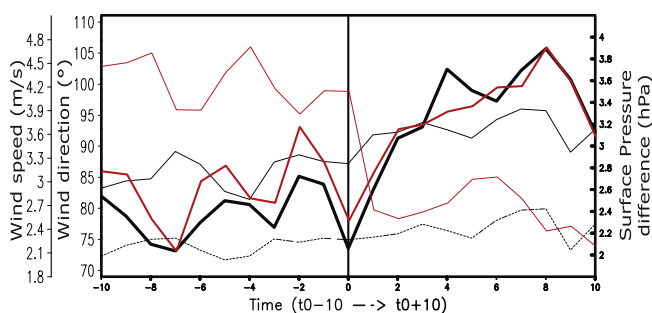
Figure 2. Red lines: Composite time series from t_0 - 10 to t_0 + 10 of the 1000 hPa wind speed (bold line) and direction (thin line) averaged over the area ( 10^\circ\text{E}–15^\circ\text{E}/22.5^\circ\text{N}–27.5^\circ\text{N} ) upstream of the Hoggar. Black lines: Composite time series of the difference between the mean sea level pressure averaged over the area ( 10^\circ\text{E}–15^\circ\text{E}/22.5^\circ\text{N}–27.5^\circ\text{N} ) upstream of the Hoggar and over the area ( 0^\circ\text{W}–5^\circ\text{E}/20^\circ\text{N}–25^\circ\text{N} ) downstream of the Hoggar (bold line); these two boxes are displayed on Figure 1; dotted line: same as thick line but for the simulation due to the Atlas alone. Thin line: same as thick line but for the simulation due to the three massifs.
