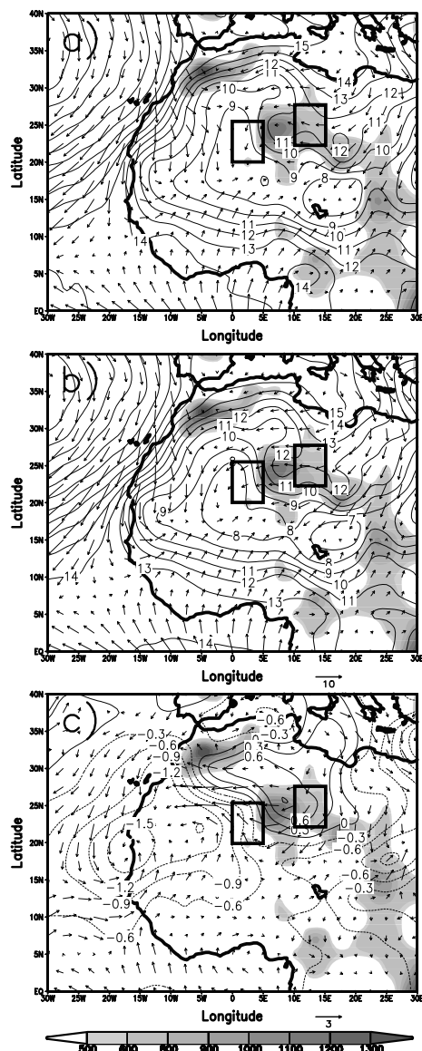
Figure 1. (a) Composite mean sea level pressure and 1000 hPa wind field (vector scale ( \text{m s}^{-1} ) is displayed below) at t_0 - 5 averaged over the period 1968–1990 by using as the reference date t_0 the ITCZ shift date for each year. Mean sea level pressure is expressed in hPa where the 1000 hPa value is subtracted. Shaded areas depict the orography of northern Africa (m). (b) Same as (a) but for t_0 + 5 . (c) Difference between (b) and (a). Boxes used for the time series of Figure 2 are plotted.
