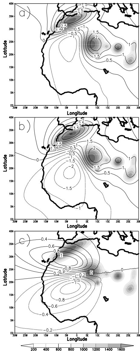
Figure 3. Surface pressure perturbation from the linear model due to the orographic effect (a) before the monsoon onset (similar to t_0 - 5 ), (b) after the monsoon onset (similar to t_0 + 5 ) and (c) the difference between (b) and (a). Shaded areas depict the idealized orography of northern Africa used in the linear model ( m ).
