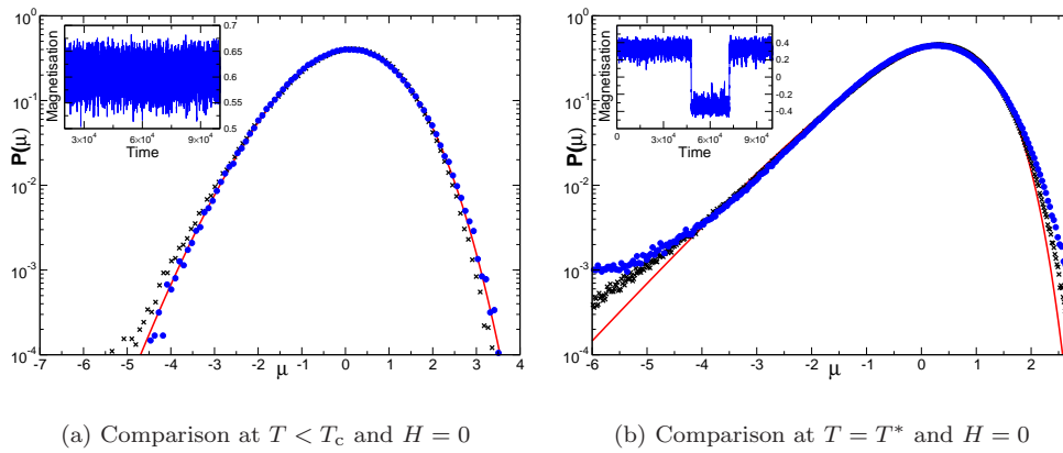
Fig. 1 – Numerical test of the Langevin dynamics, for \lambda = 2.5 and L = 65 . (a) The data ( \times ) are Monte Carlo simulations at T = 1.7 and L = 64 . The data ( \bullet ) are obtained by Langevin dynamics from equation (4) at T_{\text{dyn}} = T_c^{\text{mf}} \times 0.74 . The plain curve corresponds to the distribution of the Gaussian model ( L = 64 ) with mass M = 3.5 \times 10^{-1} [14]. (b) The plain curve is the BHP distribution [6]. The data ( \times ) are Monte Carlo simulations for L = 64 system at T^*(L) = T_c \times 0.94 [8]. The data ( \bullet ) are from the Langevin dynamics (4), at T^*(L, \lambda) = T_c^{\text{mf}} \times 0.95 . Inset: examples of magnetization dynamics.
