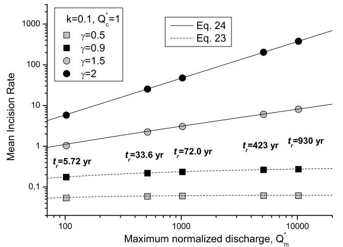
Figure 4. Evolution of mean incision rate with maximum recorded discharge Q_m^* for various local discharge exponent \gamma . Circles are obtained by numerically integrating equation (17). The return time t_r of Q_m^* gives an order of magnitude of the timescale over which incision rate is measured. When \gamma < k + 1 , the incision rate converges toward a constant value as Q_m^* increases. When \gamma > k + 1 , the long-term mean incision rate increases approximately as a power function of Q_m^* (equation (24)) with an exponent \gamma - k - 1 . See color version of this figure in the HTML.
