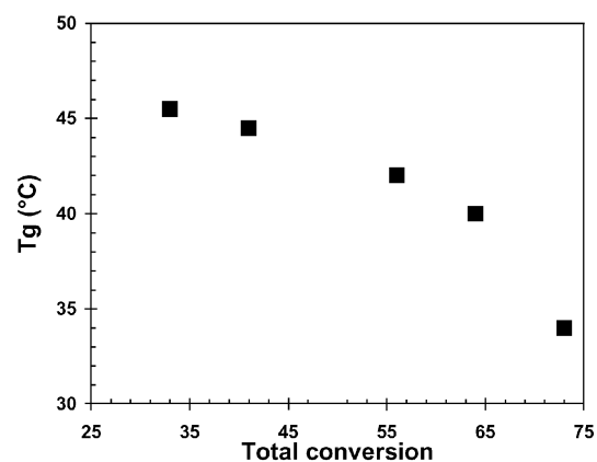
Fig. 10 Evolution of T_g of copolymer as a function of conversion ( \blacksquare : fraction f_a = 0.83 ).
