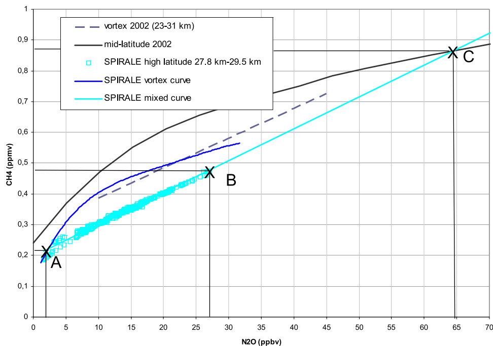
Figure 11. Same as Figure 3 in the range 0–70 ppbv for N_2O , but for the high-latitude flight in the range 27.8–29.5 km layer (clear blue squares). Correlation curves deduced from SPIRALE measurements for vortex in the ranges 23–27.8 km and 29.5–31 km layer (dark blue curve), and mixed curve in the range 27.8–29.5 km layer (clear blue curve). M1998a correlation curves for vortex conditions between 23 and 31 km (dashed gray line) and midlatitude conditions (black solid line) are shown.
