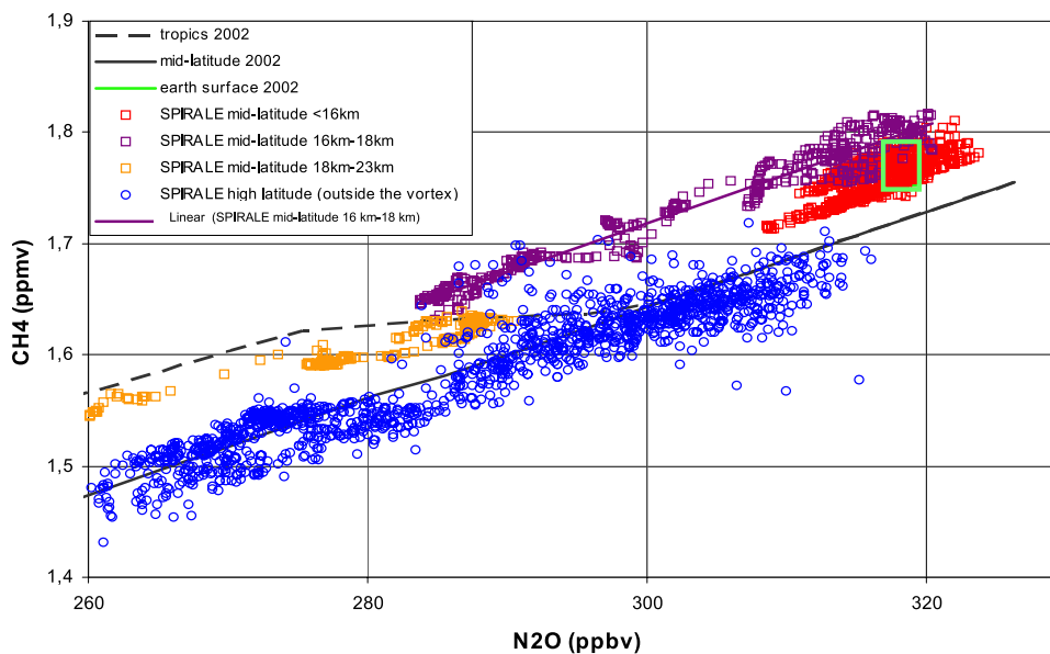
Figure 3. Detailed \text{CH}_4 : \text{N}_2\text{O} correlation values derived from SPIRALE in the range 260–330 ppbv for \text{N}_2\text{O} for the midlatitude flight: below 16 km (red squares), 16–18 km range (purple squares), 18–23 km range (orange squares), for the high-latitude flight outside the vortex (blue circles); \text{CH}_4 : \text{N}_2\text{O} correlation curves from M1998a updated for the year 2002 for midlatitudes (black solid line), and the tropics (black dashed line); 2002 Earth surface correlation from WMO [2002] (green square); and linear fit to \text{CH}_4 versus \text{N}_2\text{O} in the 16–18 km range (purple solid line).
