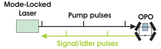
FIG. 1: Synchronously pumped OPO
