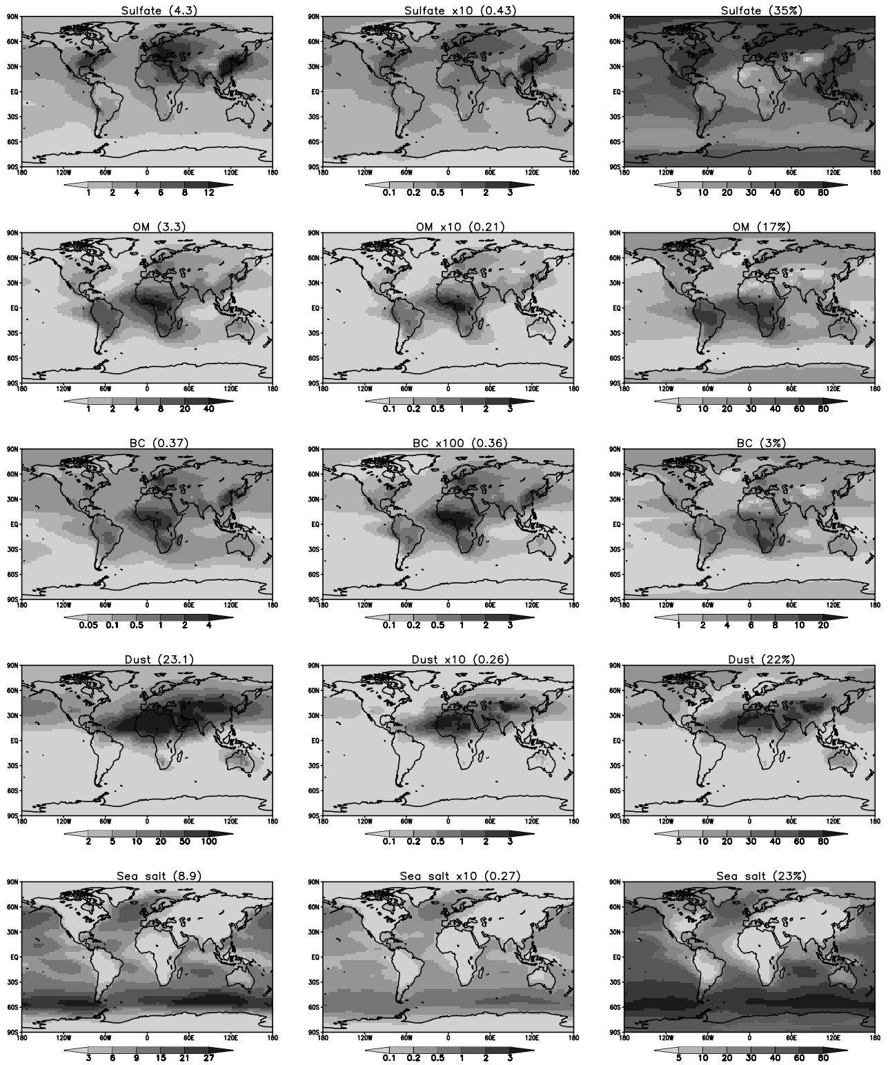
Figure 2. Distributions of annually averaged dry aerosol burden (mg m -2 , left panels), aerosol optical depth at 550 nm (dimensionless, middle panels), and contribution of individual species to total AOD at 550 nm (percent, right panels). The values in parenthesis are the global annual averages of the respective quantities. Note that scales are different on all plots. See color version of this figure in the HTML.
