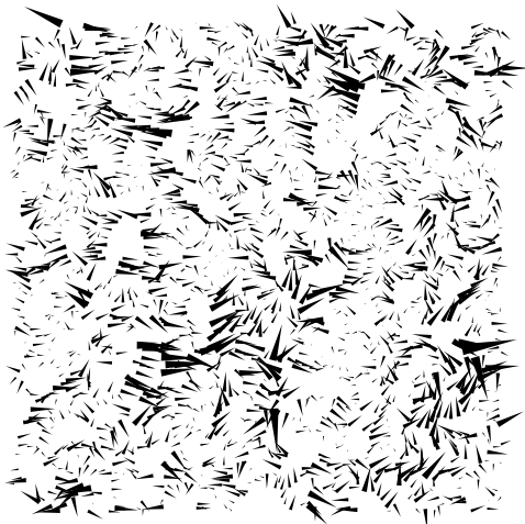
FIG. 1: Inhomogeneous part \delta\mathbf{u}(\mathbf{r}) of the displacement field \mathbf{u}(\mathbf{r}) for the imposed macroscopic uniaxial strain in elongation \epsilon_{xx} = 5.10^{-3} for a silica glass containing N = 42000 particles ( L = 83.8 Å). Projection of the field is done on the (x-z) -plane for all particles with position \mathbf{r} close to the plane, the arrow length being proportional to \delta\mathbf{u}(\mathbf{r}) . The field resides in the linear elastic regime, i.e. has a magnitude varying linearly and reversibly with the applied deformation. As visual inspection shows, it is strongly spatially correlated and involves a substantial fraction of all atoms.
