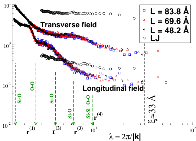
FIG. 2: (Color online) Squared amplitudes of the Fourier transforms S_L(k) and S_T(k) for the longitudinal (bottom) and transverse contributions to the normalized non-affine field \underline{\delta u}(\mathbf{r}) of silica glass at T = 0 K under macroscopic elongation, plotted vs. the wavelength \lambda = 2\pi/k (in Å). The various system sizes included demonstrate a perfect data collapse. The transverse contribution is more important for all wavelengths. The spectra become constant for large wavelengths with a relative amplitude of about 10. The spectra for a LJ glass (spheres, length given in sphere diameters) have been included for comparison [30]
