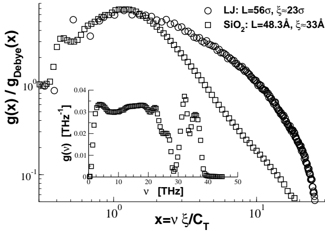
FIG. 4: Inset: VDOS g(\nu) for the silica glass at T = 300 K. Main figure: Excess of vibrational states g(x) compared to Debye's continuum model g_{Debye}(x) , using reduced units x = \nu\xi/C_T , with C_T \approx 4.2 (in LJ units) and C_T \approx 3961.4\text{m/s} for LJ and silica respectively and \xi as indicated in the figure. The Boson Peak position at x \approx 1 is well approximated by the frequency associated with the wavelength of order \xi . As expected, the peak is more pronounced for the strong glass.
