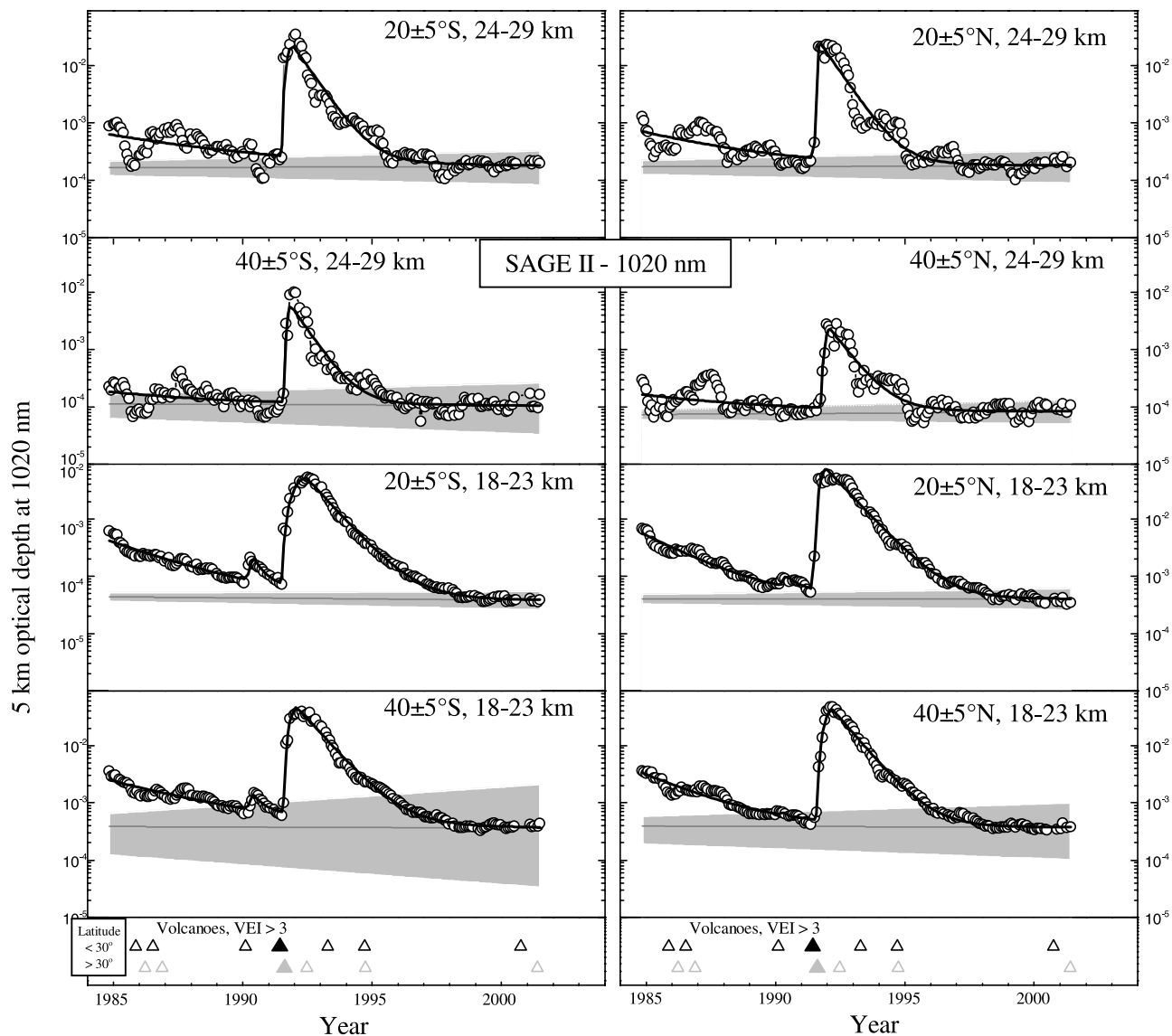
Figure 9. Optical depths integrated over two 5-kilometer altitude intervals for zonally averaged ( \pm 5^\circ ) SAGE II 1020 nm extinctions at a latitude of 20 and 40 \pm 5^\circ N/S, compared with parametric models fit to the data and with estimates of the baseline and trend for optical depth during background aerosol conditions. The estimated background is shown with \pm 95\% confidence intervals as the gray shaded area. The time of volcanic eruptions with a VEI of 4 (open triangle) and 5 (solid triangle) are shown at the bottom divided into those eruptions at latitudes less than and greater than 30^\circ of latitude.
