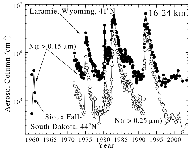
Figure 1. Aerosol columns, 16–24 km, for balloonborne in situ measurements of particles with radius > 0.15 \mu\text{m} (solid circles) above Sioux Falls ( 43.6^\circ\text{N} , 96.7^\circ\text{W} ), 1959–1960 [Chagnon and Junge, 1961], and above Laramie ( 41.3^\circ\text{N} , 105.7^\circ\text{W} ), 1971–2003 [Deshler et al., 2003]. Also included in the Laramie measurements are particles with radius > 0.25 \mu\text{m} (open circles).
