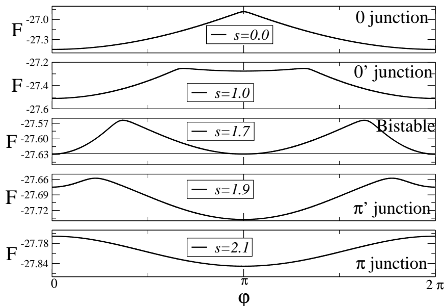
FIG. 5: The Free energy ( F ) as function of the phase difference ( \Phi ) for increasing spin from top to bottom. The \pi junction behavior is clearly seen. The other parameters are: \Delta = 1.0 , \Gamma = 4.0 , \gamma = 0 , \beta = 1000 and \epsilon = 0 .
