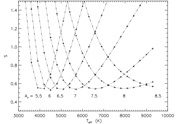
Fig. 5. Minimisation of the discrepancy between apparent and computed magnitudes, versus the blackbody effective temperature and interstellar absorption in the visible, given in magnitudes below each curve.
