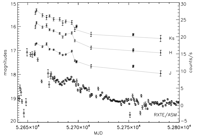
Fig. 1. Multi-wavelength XTE J1720-318 light curve. From bottom to top: Rossini-XTE X-ray light curve (indicated by diamonds); NIR J , H , and K s light curves, respectively. NIR data taken from Nagata et al. (2003) are reported with '+', and data from this paper with '*'. MJD = JD - 2400000.5
