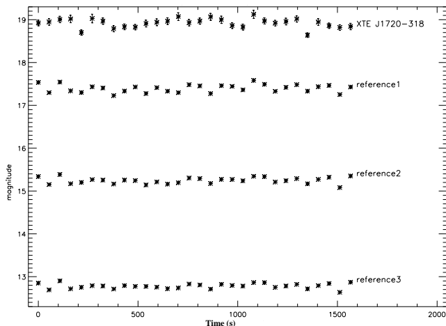
Fig. 2. Left panel: K_s light curve of XTE J1720-318 and three comparison stars of the field. Right panel: K_s light curve of XTE J1720-318 corrected from sky variations (the y-axis is in instrumental magnitude).
