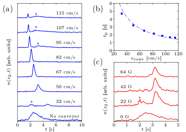
FIG. 3: (Color online). Absorption of a probe beam located at z_2 = 1.7 m from the guide entrance as a function of time t elapsed after the launch of a single atom packet, at the velocity v_i = 80 cm/s (with a rms velocity dispersion of 20 cm/s). (a): The IP traps have a depth of 50 G and a minimum field of 1 G, and one varies v_{\text{conv}} . A sharp peak of trapped atoms arrives at a time t_p . When the velocity mismatch between the conveyor and the injected atoms is too large, extra peaks corresponding to untrapped atoms appear ( \star ). (b): Arrival time t_p of the trapped atoms (squares) as a function of v_{\text{conv}} ; t_p is essentially equal to z_2/v_{\text{conv}} (dashed line). (c): The conveyor speed is fixed at 50 cm/s and one varies the IP trap depth. For too shallow traps, one gets a peak of untrapped atoms ( \star ); if the depth is too high, some atoms are reflected, which decreases the peak amplitude.
