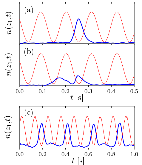
FIG. 5: (Color online). Absorption signal (thick line) measured in the conveyor belt , with a probe located at z_1 = 1 m. The IP traps have a depth of 32 G, and one has v_{\text{conv}} = v_i = 88 cm/s. The thin line is the measured B_z field component produced by the conveyor. (a): Proper synchronization of the launching of one packet to load a single trap (the cloud arrives in coincidence with a potential minimum). (b): The launching occurs at a time \Lambda/(2v_{\text{conv}}) before, resulting in a splitting of the cloud into two consecutive traps. (c): Multiple injection of packets, with the proper synchronization to load one every second trap.
