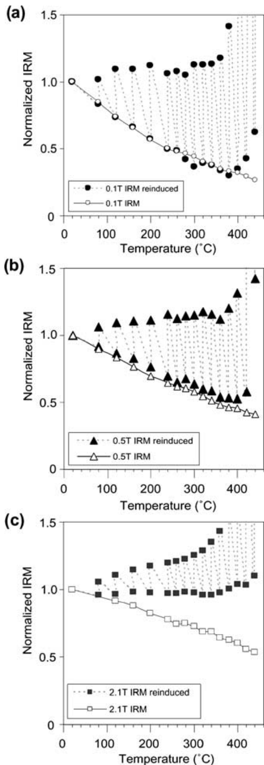
Figure 4. Results of thermal demagnetization under an argon atmosphere of paired samples after heating to 250 °C for 22 hr, using the method of Van Velzen & Zijdeveld (1992) (see text for details). Circles, triangles and squares correspond respectively to 0.1 T IRM (a), 0.5 T IRM (b) and 2.1 T IRM (c). Open symbols correspond to IRM induced only once (reference sample) and full symbols correspond to IRM reinduced after each demagnetization step.
