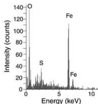
Figure 3. Microscopic observations on heated samples. (a) SEM image showing a pyrite crystal in the matrix of claystone; white stars locate the EDS analysis. (b) SEM image, showing a pyrite crystal in a reddened pyrite aggregate (>1 mm in size); white stars locate the EDS analysis.
