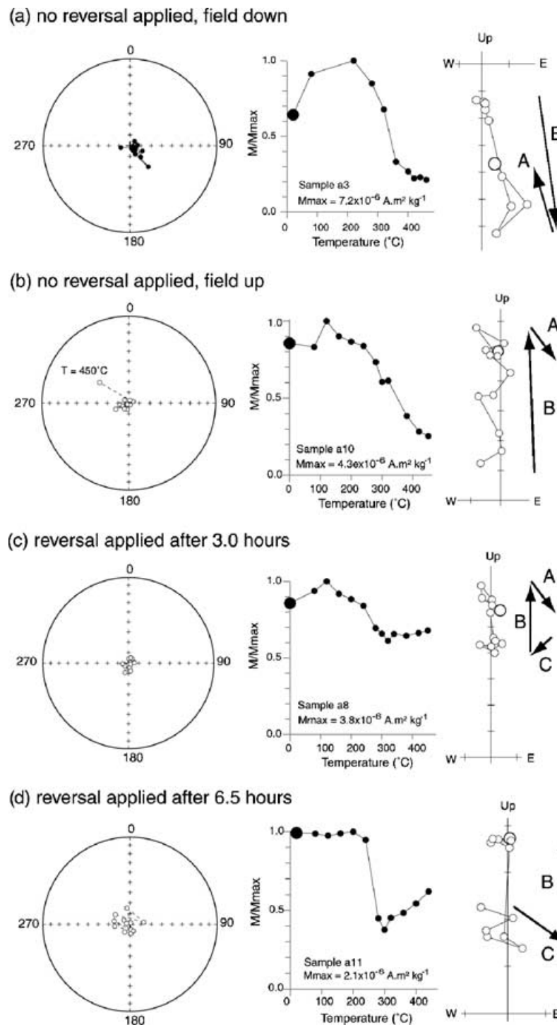
Figure 6. Results of thermal demagnetization under an argon atmosphere for experiments with one polarity (a and b) and experiments with two polarities (c and d). Same convention as for Fig. 5.
