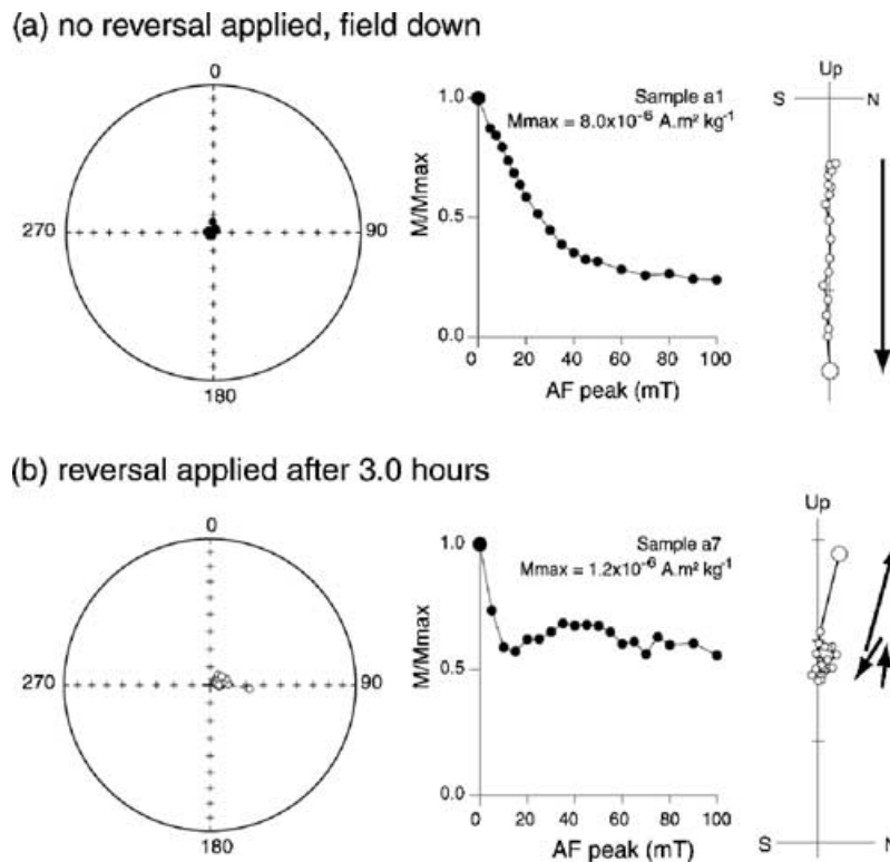
Figure 5. AF demagnetization results for experiments with one polarity (a) and two polarities (b): stereoplots, intensity plots, Zijderveld diagrams and their interpretation.
