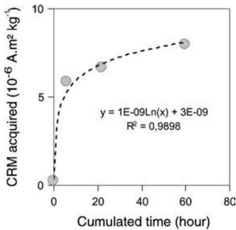
Figure 2. CRM acquired versus cumulative heating time at 250 °C for sample a1. The dashed line indicates the trend of change with time.
