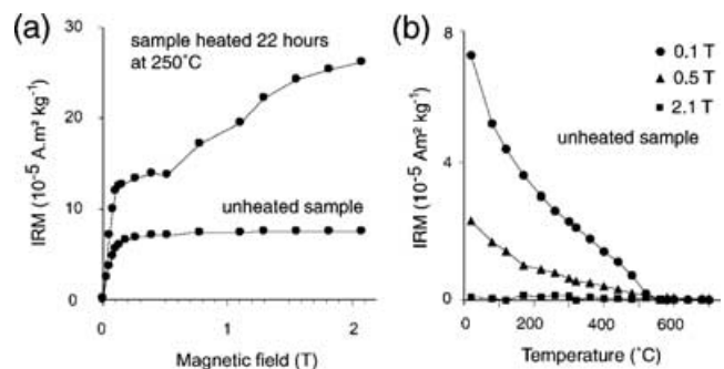
Figure 1. (a) Acquisition of IRM at room temperature for a representative unheated sample and for a representative heated sample. (b) Stepwise thermal demagnetization of a three-axis IRM imparted on an unheated sample, following the method of Lowrie (1990). Circles, triangles and squares correspond to soft (0.1 T), medium (0.5 T) and hard (2.1 T) magnetic components, respectively.
