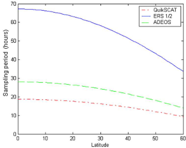
Figure 1 Indicative sampling period of different scatterometers in function of the latitude.
