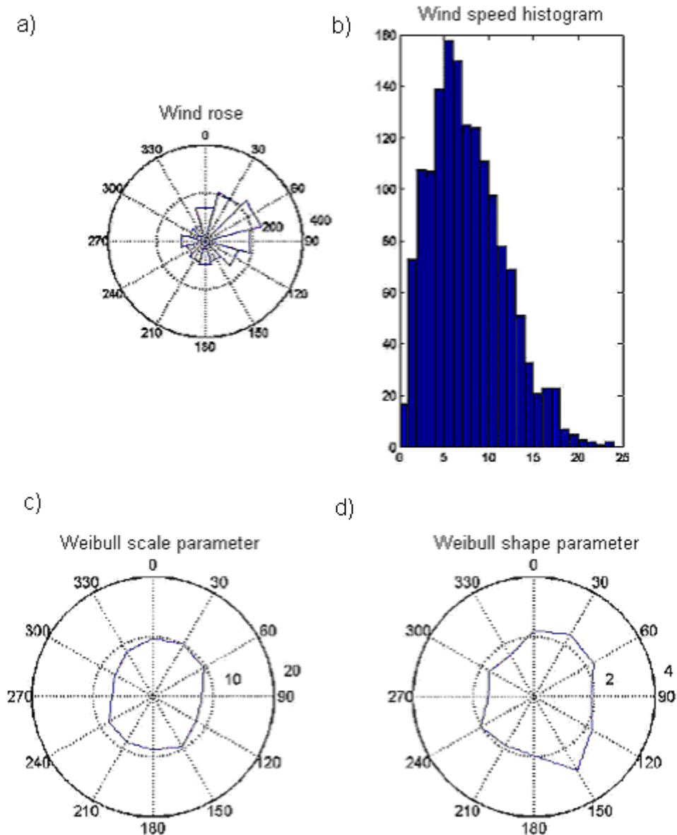
Figure 3 Wind statistics using data acquired by Quikscat between 1999 and 2001: a) Wind rose showing the number of measurements in each direction sector b) Wind speed histogram with speed bins of 1 m/s c) Weibull scale parameter computed for each direction sector d) Weibull shape parameter computed for each direction sector.
