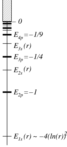
Figure 1: Energy of the bound states of the exciton. Energies are expressed in multiples of the effective Rydberg of the exciton.
