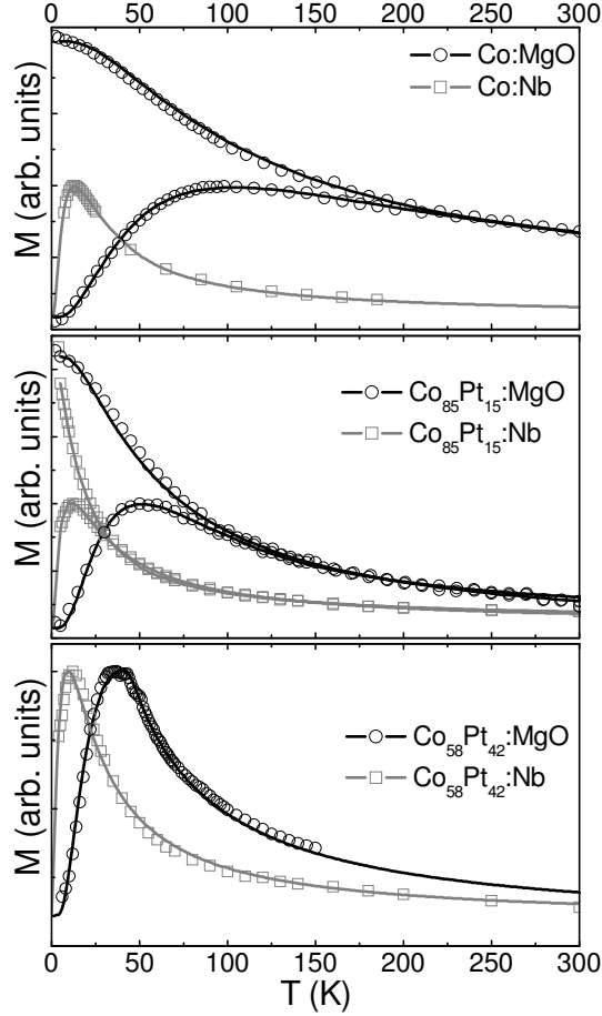
FIG. 3: ZFC-FC curves measured on the Co, \text{Co}_{85}\text{Pt}_{15} and \text{Co}_{58}\text{Pt}_{42} clusters embedded in MgO and Nb matrices. The curves were recorded in a small field of 5 mT (Co:MgO and \text{Co}_{85}\text{Pt}_{15} :MgO) or 10 mT (Co:Nb, \text{Co}_{85}\text{Pt}_{15} :Nb, \text{Co}_{58}\text{Pt}_{42} :Nb and \text{Co}_{58}\text{Pt}_{42} :MgO). The dots correspond to the measurements and the continuous lines correspond to the fits using the model described below.
