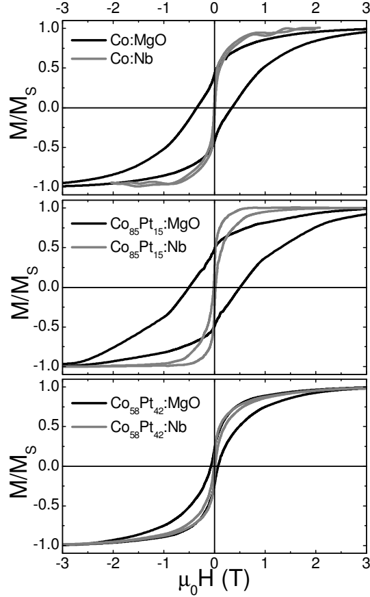
FIG. 2: Normalized hysteresis loops measured at T = 10 K on the samples with Co, \text{Co}_{85}\text{Pt}_{15} and \text{Co}_{58}\text{Pt}_{42} clusters. The dark lines correspond to the measurements in the MgO matrix and the grey lines correspond to the measurements in the Nb matrix.
