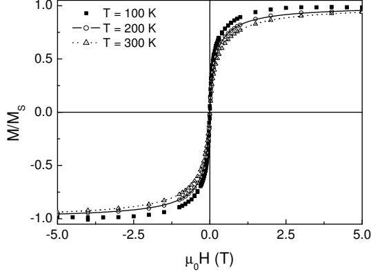
FIG. 4: Superparamagnetic M(H) curves measured on the Co:MgO sample at 100 K, 200 K and 300 K. The two measures at the highest temperatures are fitted using the convolution of a Langevin function with Log-normal distribution of the magnetic diameter. The curve recorded at 100 K cannot be fitted with the same parameters due to a non negligible MAE.
