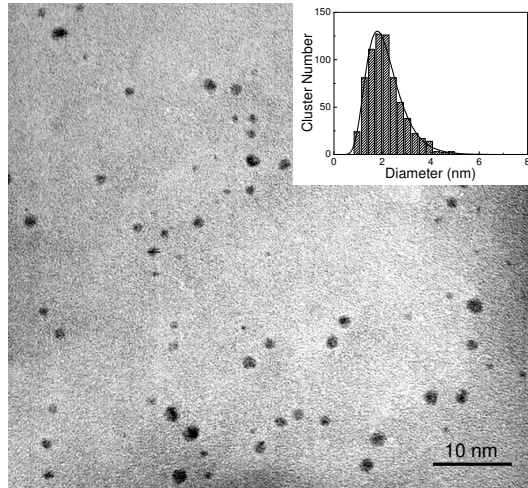
FIG. 1: TEM micrograph of the \text{Co}_{85}\text{Pt}_{15} clusters deposited on an amorphous carbon grid. Inset: diameter distribution. The histogram corresponds to the TEM measurements and the continuous line corresponds to a Log-normal fit.
