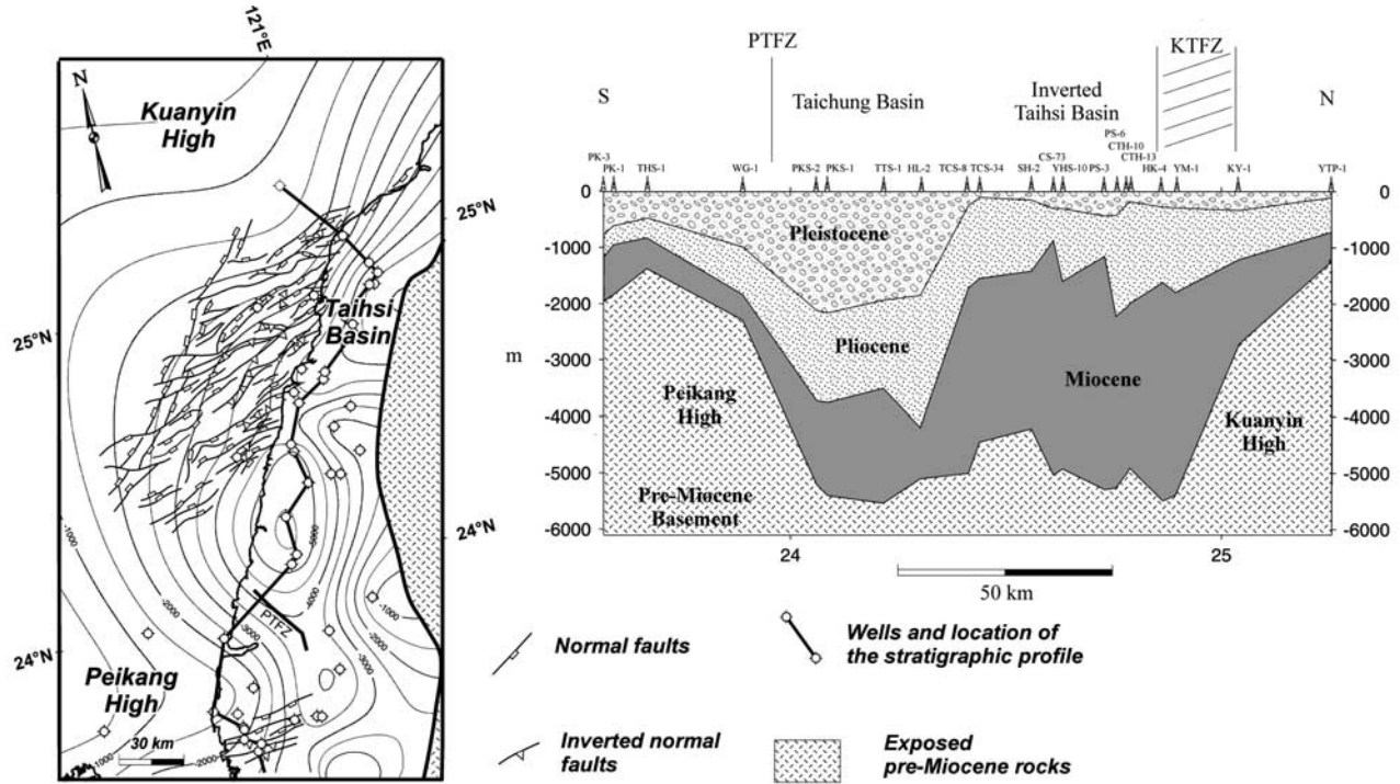
Figure 4. (a) Contoured map of pre-Miocene rocks (“basement”) and main structural pattern of offshore Taiwan. Contour interval is 500 m. PTFZ-Pakua transfer-fault zone, KTFZ-Kuanyin transfer fault zone discussed in the present work. (b) Along-strike stratigraphic profile of the Taiwan foreland showing the location of basins and highs. Note the major basement highs (Kuanyin high and Peikang high) and the inverted Taihsi Basin located on the southern edge of the Kuanyin high. The Pakua transfer fault zone delineates the Peikang high from the northern Paleogene-Neogene basins (Taichung and Taihsi basins).
