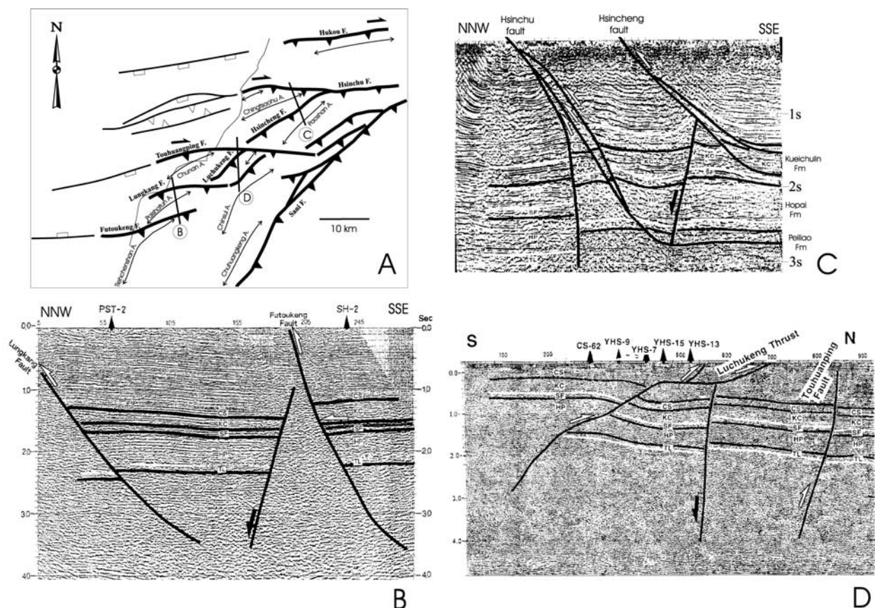
Figure 5. (a) Detailed structural map of the Hsinchu area (location in Figure 2). (b, c, and d) Seismic reflection profiles (location in Figure 5a) after Yang et al. [1996] (Figures 5b and 5c) and Yang et al. [1997] (Figure 5d). Letters on profiles refer to names of formations of the stratigraphic column of Figure 6.
