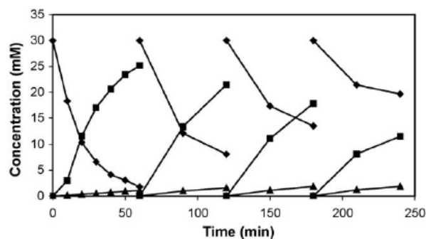
Fig. 2. Biotransformation of benzonitrile (30 mM; ◆) into benzamide (■) and benzoic acid (▲) by immobilized Rhodococcus equi A4. See Section 2 for details.
