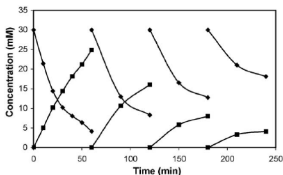
Fig. 4. Biotransformation of ( R,S )-3-hydroxy-2-methylene-3-phenylpropanenitrile (30 mM; \blacklozenge ) into ( R,S )-3-hydroxy-2-methylene-3-phenylpropanamide ( \blacksquare ) by immobilized Rhodococcus equi A4. See Section 2 for details.
