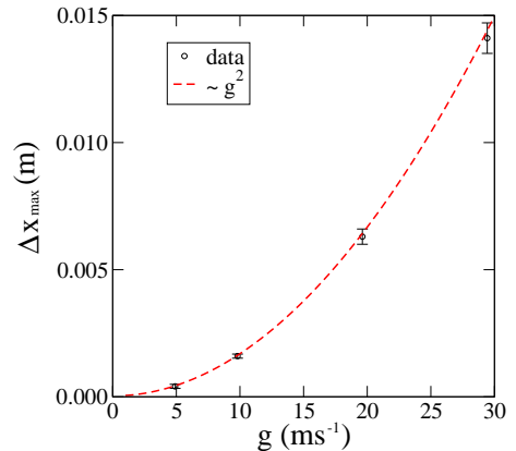
FIG. 19: Scaling of the maximum displacement \Delta x_{max} with gravity g .
