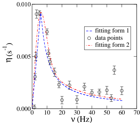
FIG. 21: The compaction rate \eta as a function of the frequency (circles) fitted by two different functions; see text. \nu
