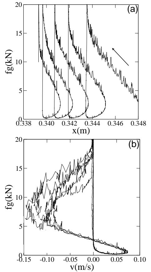
FIG. 5: Force f_g exerted by the grains on the free wall as a function of displacement x (a) and the velocity v (b). (
