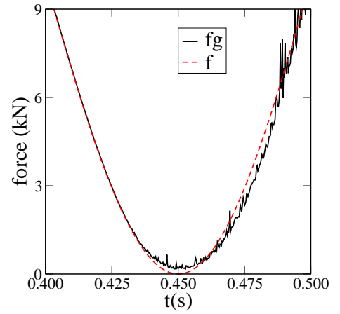
FIG. 4: The force f_g exerted by the grains and the driving force f on the free wall as a function of time t .
