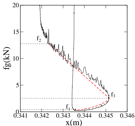
FIG. 9: Variation of the packing reaction force f_g with displacement x over one period (full line) and an approximate fitting form (dashed line).
