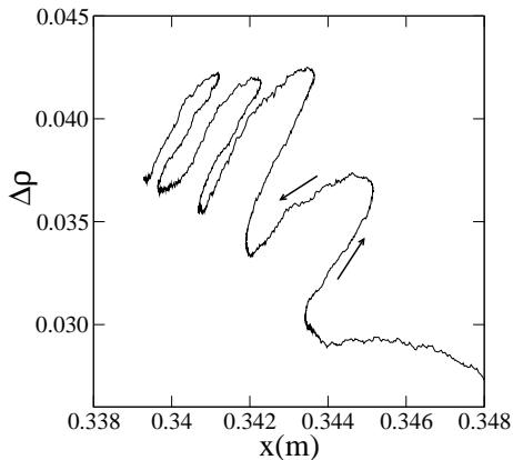
FIG. 15: Variation \Delta\rho of the solid fraction from the initial state as a function of the displacement x of the free wall.
