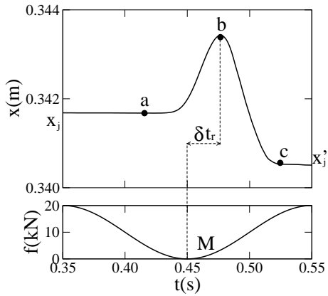
FIG. 3: A zoom on a single period; see Fig. 2.
