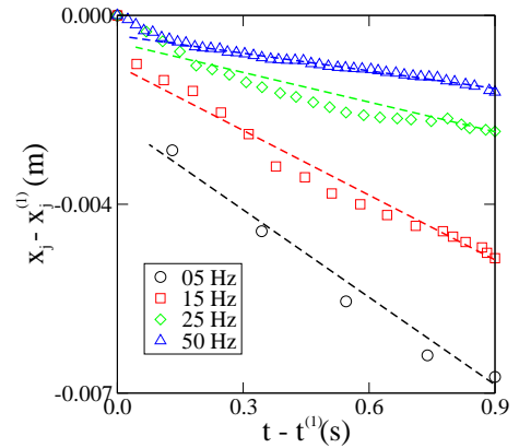
FIG. 14: Evolution of the jamming position x_j from the position x^{(1)} reached at t = t^{(1)} = 0.1 s for four different frequencies.
