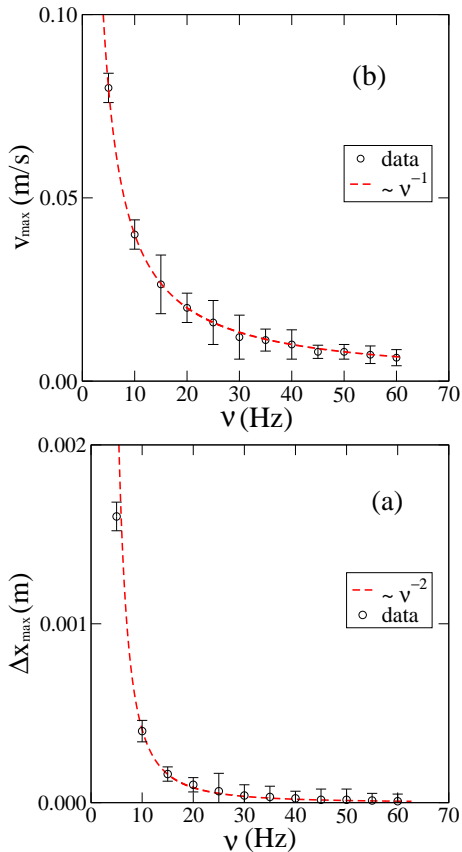
FIG. 17: Maximum displacement \Delta x_{max} (a) and the maximum velocity v_{max} (b) as a function of the frequency \nu .
