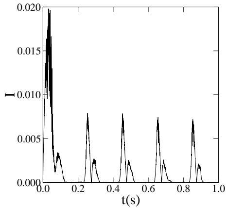
FIG. 8: The evolution of the inertia number I over five periods.
