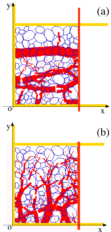
FIG. 7: Normal forces in the passive (a) and active (b) states. Line thickness is proportional to the force.
