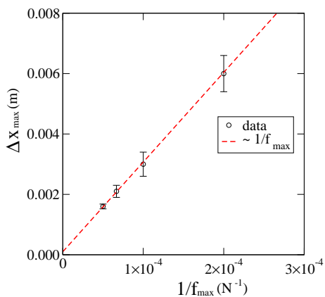
FIG. 18: Scaling of the maximum displacement \Delta x_{max} with the force amplitude f_{max} .
