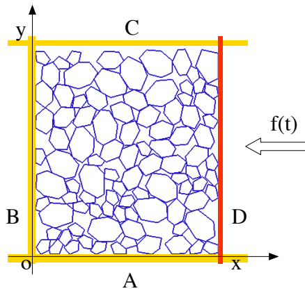
FIG. 1: The geometry of the packing.
