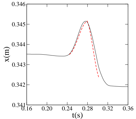
FIG. 10: Displacement x of the free wall as a function of time (full line) and analytical fit from the phenomenological model (dashed line).
