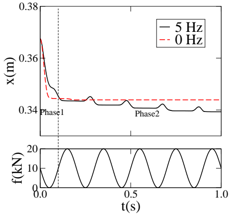
FIG. 2: The evolution of the displacement x of the free wall (up) in response to harmonic loading (down).
