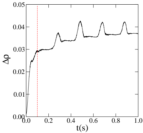
FIG. 13: Evolution of the solid fraction \Delta\rho from the initial state as a function of time over several periods.
