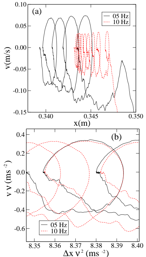
FIG. 16: Phase space trajectories for two frequencies without scaling (a) and with scaling (b) of the displacements and velocities.
