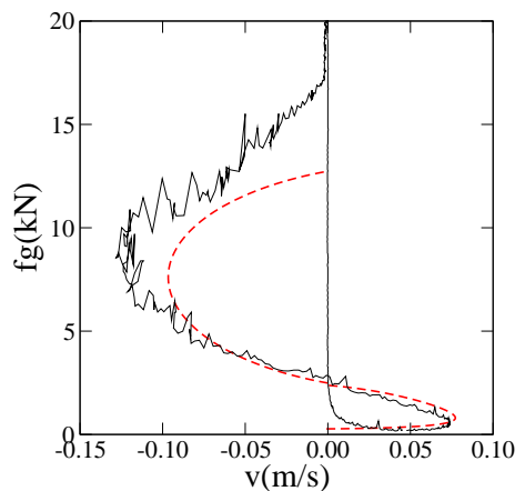
FIG. 11: Force f_g exerted by the grains on the free wall versus velocity v over one period (full line) and analytical fit from the phenomenological model (dashed line).
