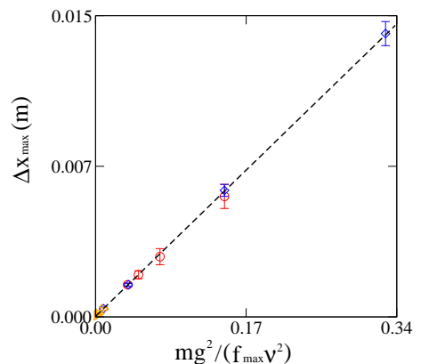
FIG. 20: Scaling of the maximum displacement \Delta x_{max} with loading parameters from simulations with different values of the frequency \nu (squares), the force amplitude f_{max} (circles) and the gravity g (diamonds).
