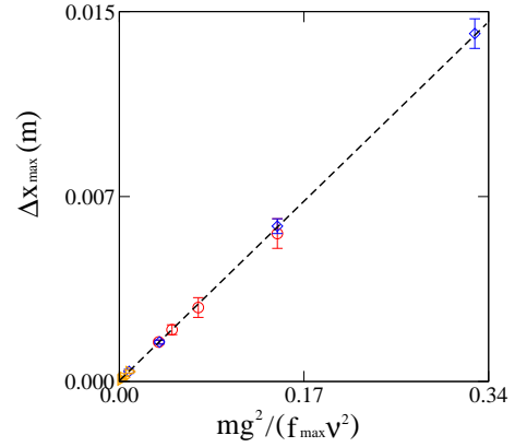
FIG. 20: Scaling of the maximum displacement \Delta x_{\max} with loading parameters from simulations with different values of the frequency \nu (squares), the force amplitude f_{\max} (circles) and the gravity g (diamonds).
