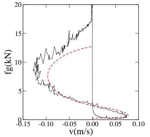
FIG. 11: Force f_g exerted by the grains on the free wall versus velocity v over one period (full line) and analytical fit from the phenomenological model (dashed line).
