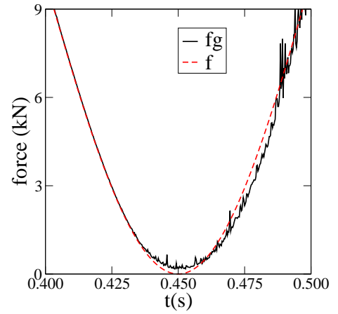
FIG. 4: The force f_g exerted by the grains and the driving force f on the free wall as a function of time t .
