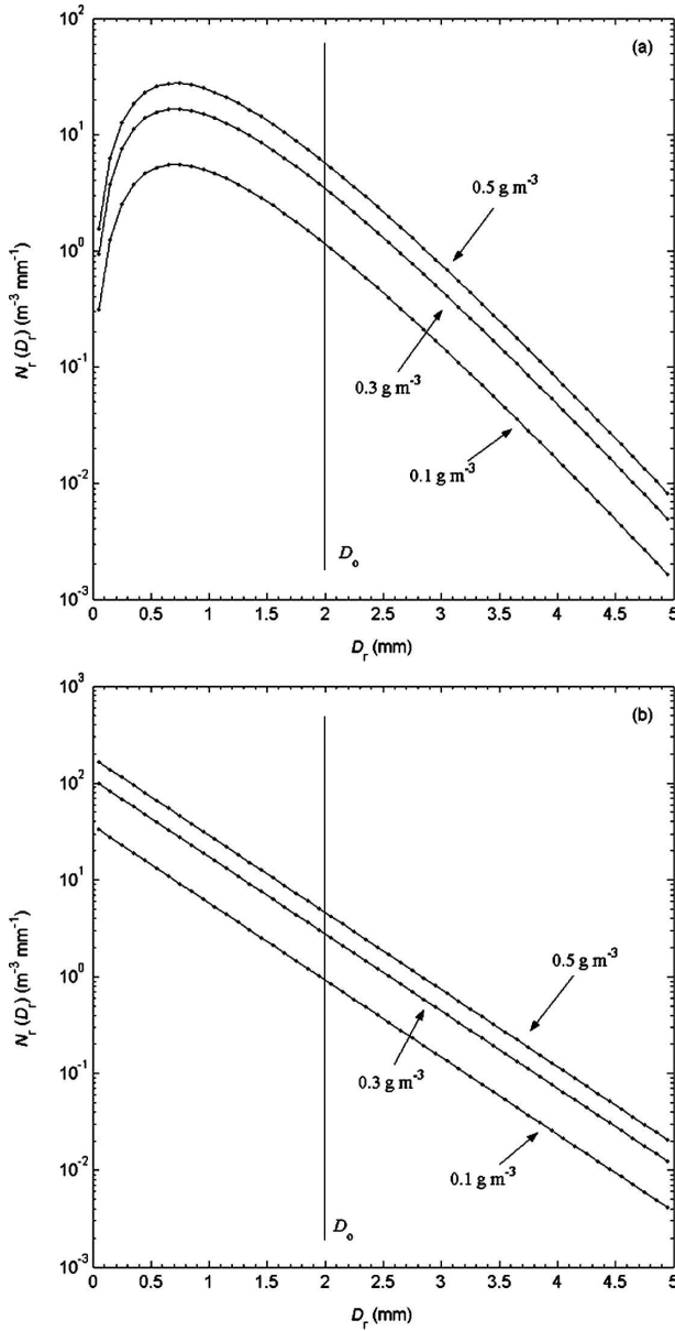
FIG. 4. RDSD represented by a gamma distribution. RDSD is displayed for three values of the rainwater content and for a median diameter D_0 fixed at 2 mm (represented by the black vertical line). Here, D_r is the raindrop diameter and N_r the volumic concentration per diameter class. RDSD with (a) \mu = 2 and (b) \mu = 0 .
