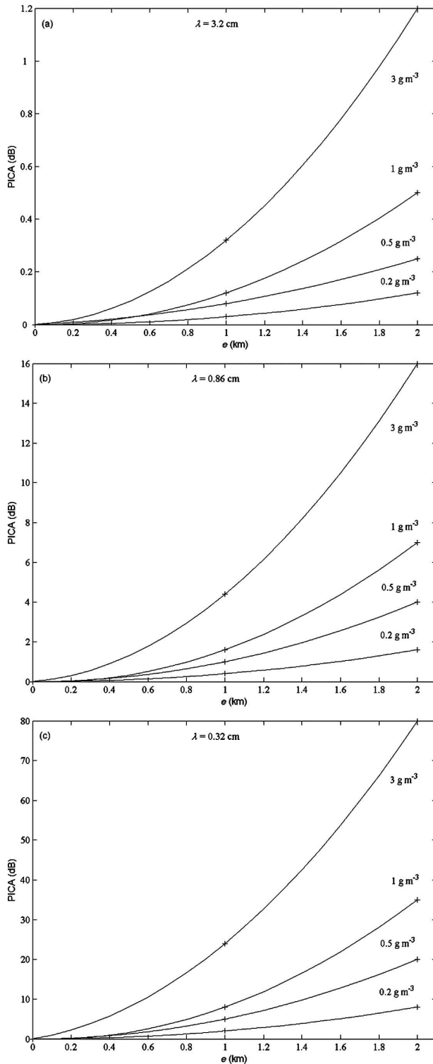
FIG. 16. Maximum value of PICA (dB) with respect to cumulus thickness e (km) according to cloud maximum liquid water content ( M_c^{\text{max}} = 3, 1, 0.5, and 0.2 \text{ g m}^{-3} ); cloud shape factor is 5. Wavelengths of observations are (a) 3.2, (b) 0.86, and (c) 0.32 cm.
