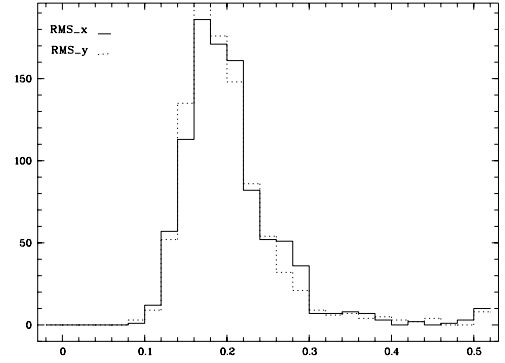
Fig. 8. Histogram of rms of plates reductions in right ascension and declination expressed in ″. The associated mean values are: \varepsilon_{O-C,x} = 0''.21 \pm 0.07 , \varepsilon_{O-C,y} = 0''.19 \pm 0.07 and \sqrt{\varepsilon_{O-C,x}^2 + \varepsilon_{O-C,y}^2} = 0''.28 \pm 0.08 .
