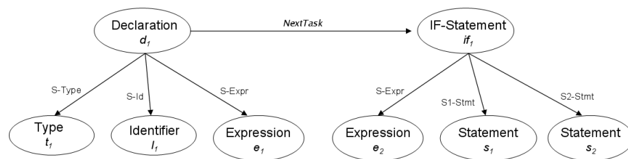
Figure 7: An example of source program encoding
