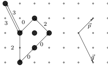
Fig. 8. The salient-word of this Q-convex set (3200203) has an odd size
