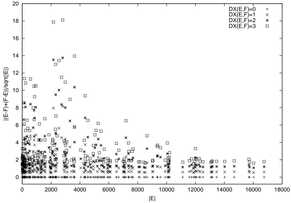
Fig. 4. An upper bound to \frac{\text{card}(E \triangle F)}{\sqrt{\text{card}(E)}} for the 184 generated Q-convex sets
