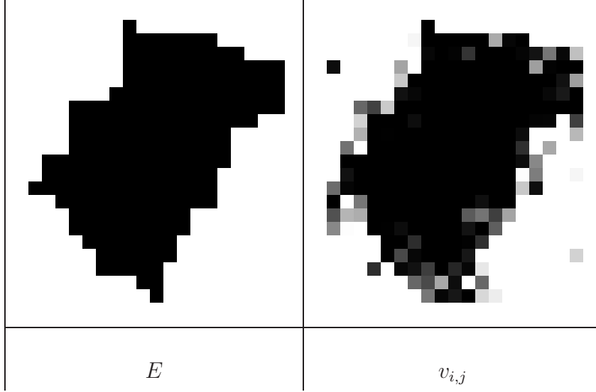
Fig. 2. A Q-convex set E and the corresponding extremal values of v_{i,j} for e = 3 . In this case we have \text{card}(E) = 200 and \sum_{(i,j) \in E} (1 - v_{i,j}) + \sum_{(i,j) \in E^c} v_{i,j} = 33.7 .
