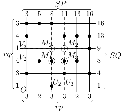
Figure 10: Median points and lines of a discrete set according to Manhattan distance.
