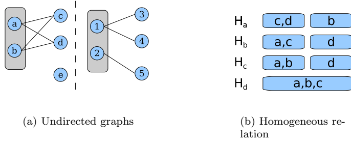
Figure 1: (a) Modules and umodules in a graph: \{a, b\} is a module and also a umodule, \{1, 2\} is a umodule but is not a module. (b) A homogeneous relation with a module which is not a umodule. \{a, b\} is a module: they belong to the same equivalence class in both H_c and H_d . \{a, b\} is not a umodule: c and d belong to the same class in H_a , and to different classes in H_b .
