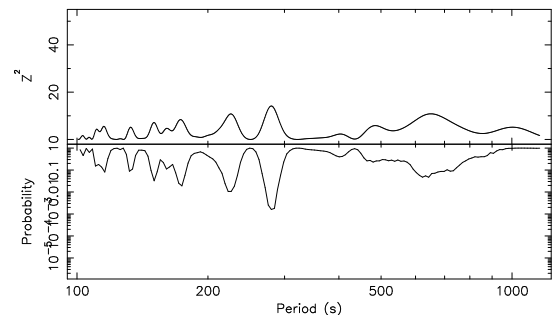
FIG. 3.— Flare of 2002 October 3: Z^2 -periodogram and associated probabilities derived from MC simulations of 500 event lists. Total flare duration is \sim 3000 s and period range spans 100–1000 s. No significant peaks are detected
