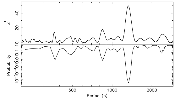
FIG. 2.— Flare of 2004 August 31: Z^2 -periodogram and associated probabilities derived from MC simulations of 10^6 event lists. Total flare duration was \sim 9000 s and thus the period range is 100–3000 s. The peak is at P = 1330 s and rises to a Z^2 value of 46, and has an associated probability of \sim 10^{-6} .
