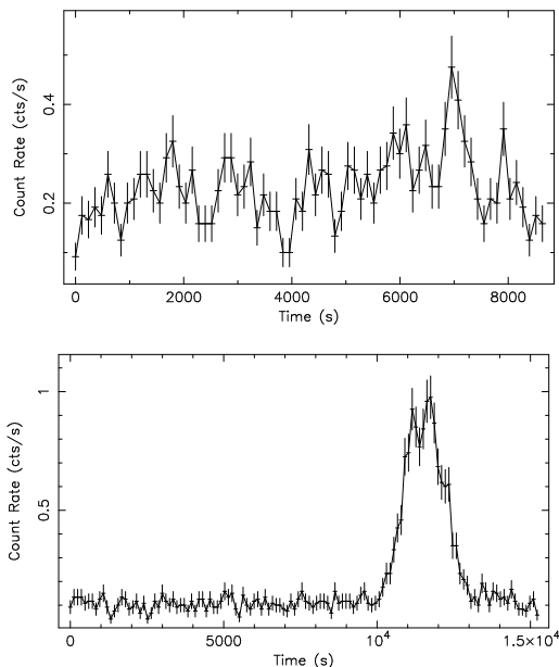
FIG. 1.— Top panel : Light curve of the 2004 August 31 flare ( T \sim 9 ks). Bottom panel : Light curve of complete \sim 15 ks 2002 October 3 observation. Resolution is 120 s.
