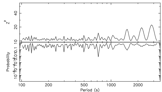
FIG. 4.— Data of 2002 October 3 before flare: Z^2 -periodogram and associated probabilities derived from MC simulations of 500 event lists. Total duration of observation is \sim 10000 s and period range spans 100–3000 s. No significant peaks are detected
