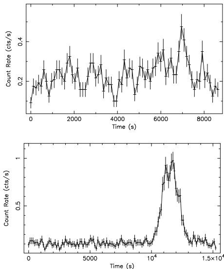
FIG. 1.— Top panel : Light curve of the 2004 August 31 flare ( T \sim 9 ks). Bottom panel : Light curve of the whole \sim 15 ks 2002 October 3 observation of Sgr A*. Resolution is 120 s.
