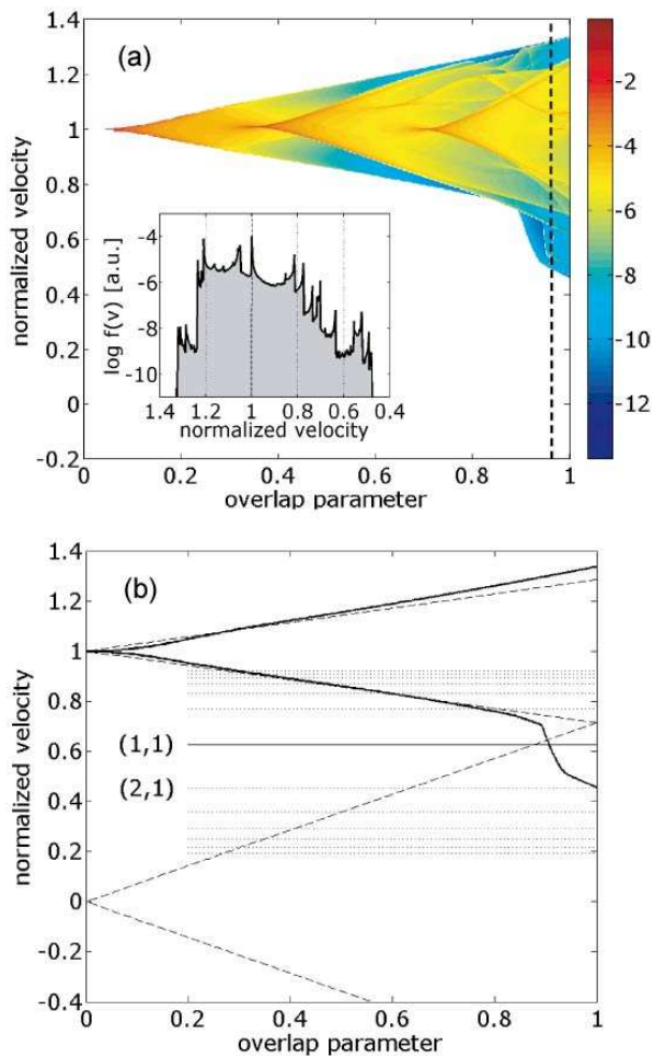
FIG. 8: Numerical devil's staircase. a) Probability distribution function f(v) (with logarithmically scaled color coding) of the velocity for the dynamics of Fig. 6, as a function of overlap parameter s = 2.8\sqrt{\varepsilon} after a time \tau = 12\pi , i.e. 10 Poincaré stroboscopic periods (inset, f(v) for the value of s indicated by the vertical dashed line). b) Velocity frontiers of f(v) versus s for t = 12\pi ; dashed oblique lines starting from v = 0 and v = 1 indicate the primary resonances trapping domains; secondary resonances (n, m) are indicated at rational velocities mk/(n + mk) .
