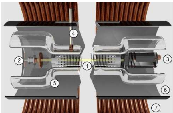
FIG. 1: Travelling Wave Tube rendering: (1) helix, (2) electron gun, (3) trochoidal analyzer, (4) antenna, (5) glass vacuum tube, (6) slotted rf ground cylinder, (7) magnetic coil.
