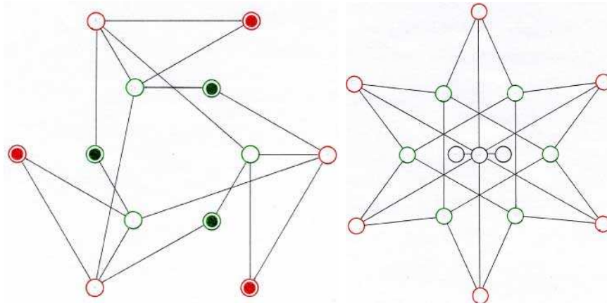
Figure 2: A schematic illustration of the fine structure of the inner ( left ) and outer ( right ) shells of the projective line \text{PR}_{\Delta}(1) , where any two distant points are joined by a line segment. In both the cases, the two sets of points are distinguished by different colours; in the former case, in addition, the filled circles denote the ‘fat’ points and in the latter case also the nucleus (three points in the center, the middle one being W ) and its relation to the shell in question are shown.
