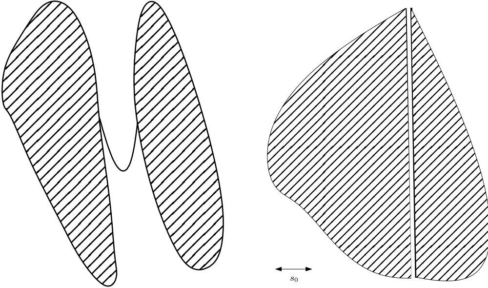
Figure 1: One single 0-connected component that is not r_0 -standard for any r_0 (left). This set has two r_0 -connected components at scale 0 but one at scale s_0 > 0 (right).
