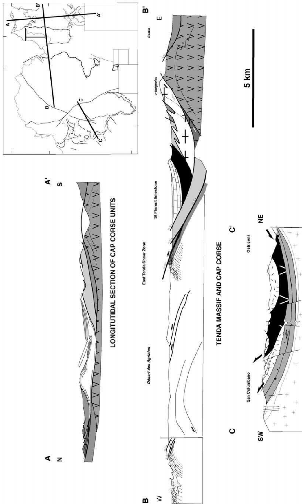
Figure 4. Same as Figure 3 but cross sections of Alpine Corsica.
