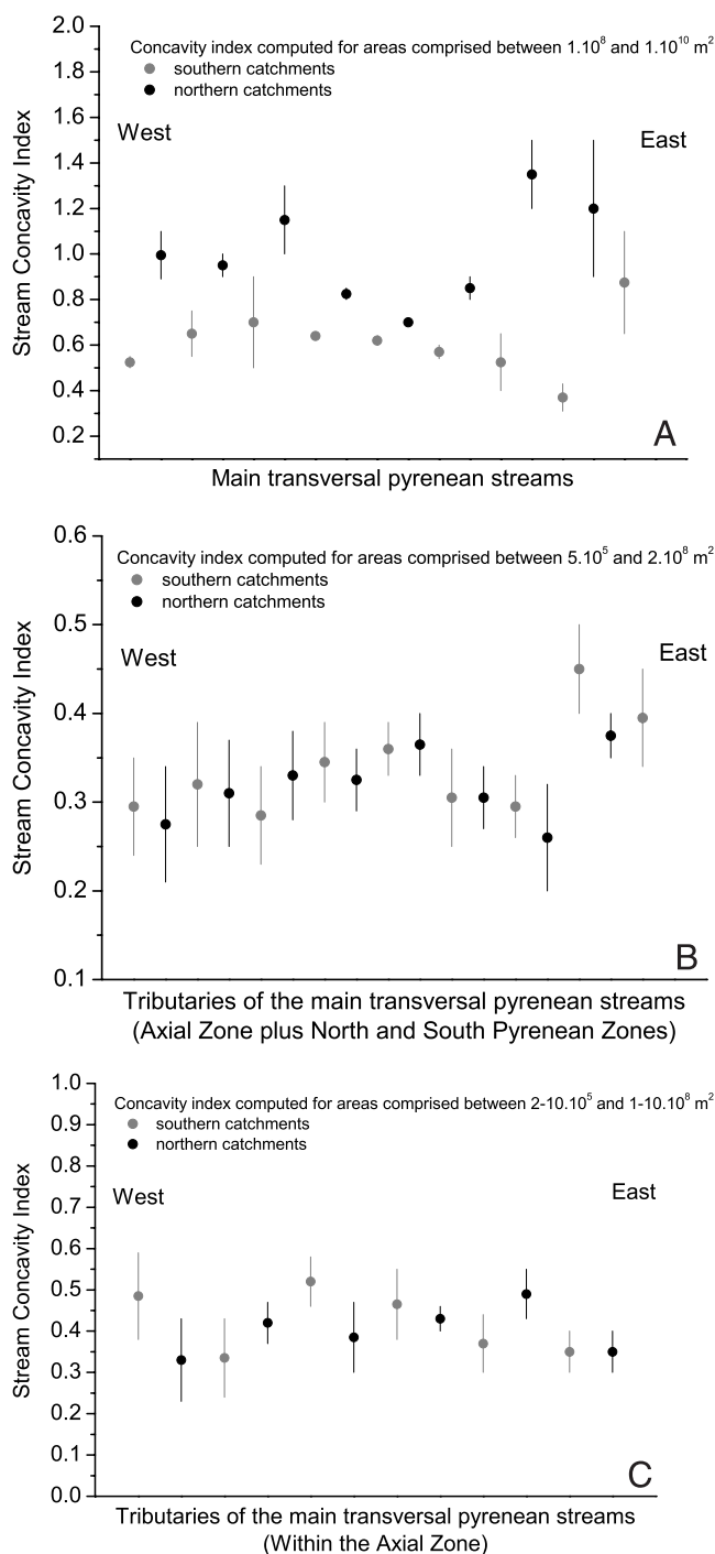
Figure 9. Concavity profiles of the main transverse rivers and their tributaries. Using the slope area relationship we computed the concavity indices for all the mainstreams and their tributaries. (a) The drainage area and local slope value along the main transversal streams were computed using the steepest-slope criteria. The concavity index analysis shows the higher concavity for the northern flank main rivers, that is, for drainage area values higher than 10^8 \text{ m}^2 . (b) The concavity index of all the tributaries is determined by analyzing the slope variation for drainage areas ranging from 5 \times 10^5 \text{ m}^2 to 10^8 \text{ m}^2 within the whole area covered by the main drainage basins drawn in Figure 7. The main basin outlets correspond to the morphological fronts of the north and south Pyrenean zones. (c) Subbasins concavity indexes have been performed for parts of the main basins located within the Axial Zone. Whatever their location on the northern or on the southern flank of the Pyrenees, the tributaries have a similar concavity index. Figure 9c shows that the concavity indexes are higher in the high chain than in the rest of the range.
