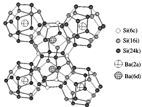
FIG. 3. Structure of Si_{20} and Si_{24} cages and the Ba atoms in Ba_8Si_{46} .
