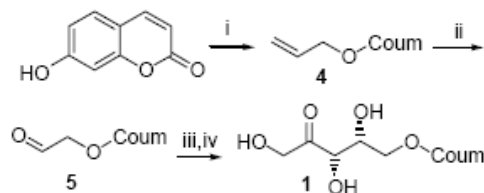
Scheme 4. Synthesis of 1 : (i) \text{CH}_2=\text{CH}-\text{CH}_2\text{Br} , \text{K}_2\text{CO}_3 , ( 4 , 96%); (ii) \text{O}_3 , \text{Me}_2\text{S} , ( 5 , 62%); (iii) RAMA, DHAP, mCD; (iv) acid phosphatase, ( 1 , 35% overall for the last two steps).
