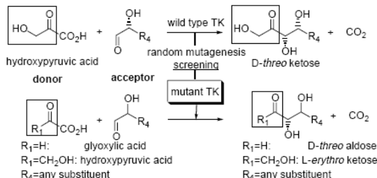
Scheme 3. Access to new D-threo -aldoses or L-erythro -ketoses by TK engineering.
