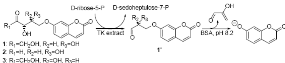
Scheme 2. Fluorescence assay based on umbelliferone release.
