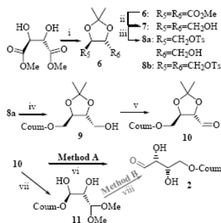
Scheme 5. Synthesis of 2 : (i) (CH 3 ) 2 C(OCH 3 ) 2 ( 6 , 85%); (ii) NaBH 4 ( 7 , 73%); (iii) TsCl, NaOH ( 8 , 83%); (iv) Coum-OH, NaH ( 9 , 71%); (v) Dess–Martin periodinane ( 10 , 49%); (vi) Dowex H + resin ( 2 , 25%); (vii) Dowex H + resin ( 11 , 43%); (viii) Dowex H + resin ( 2 , 28%).
