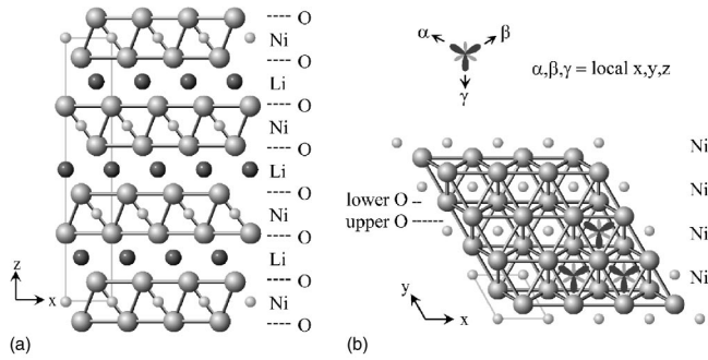
FIG. 1. (a) A side view of \text{LiNiO}_2 structure ( R\bar{3}m ) revealing stacks of \text{NiO}_2 slabs and Li layers. The thin solid lines connecting four Ni sites denote the boundary of a unit cell. (b) A top view of a \text{NiO}_2 slab showing the network of edge-shared octahedra. At the right bottom corner, the threefold arrangement of Ni 3d_{\alpha^2-r^2/3} ( \alpha = x, y, \text{ or } z ) orbitals is also shown.
