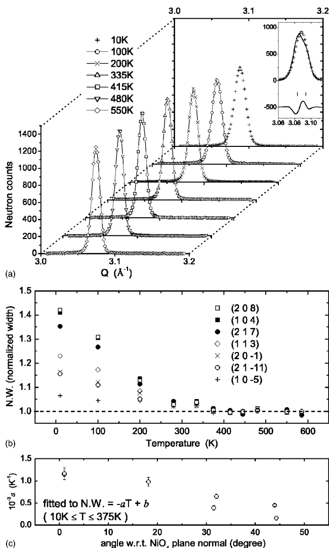
FIG. 3. (a) Temperature-dependent peak broadening observed for the (1 0 4) reflection of the neutron-diffraction profile of \text{LiNiO}_2 . The inset is the comparison between the measured profile at 10 K and the calculated one based on C2/m space group. (b) The normalized peak widths of the reflections in the neutron diffraction profiles of \text{LiNiO}_2 obtained by Gaussian fitting. The obtained peak widths at each temperature were normalized to the average of those beyond 400 K. (c) The slope of the temperature-dependent peak widths as a function of the angle between the momentum vector and Ni—O bond direction.
