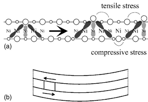
FIG. 11. (a) A lateral view of a single \text{NiO}_2 slab. Double-sided lobes are \text{Ni } 3d_{2-2/3} orbitals with long \text{Ni}-\text{O} bonds, and empty circles are oxygen sites. For either oxygen or nickel site, those closer or farther from the viewer are represented by relative sizes. For \text{Ni}^{3+} orbitals, black and gray lobes denote closer and farther positions, respectively. (b) A lateral view of a stack of multiple slabs. The arrows indicate the direction of monoclinic shear. The dotted line is the domain boundary, beyond which the curvature reverses.
