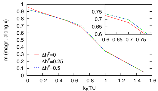
Figure 2: (color online) Results of the Monte-Carlo simulation for the classical 2D- XY model in a 200 \times 200 lattice. The Inset is a magnetification of the main figure close to T = 0.7J/k_B .
