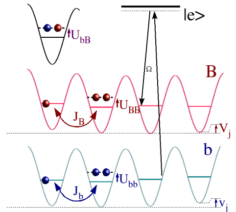
Figure 3: (color online) Atomic level scheme of a two-component Bose mixture in a random optical lattice used to design spin models in random magnetic fields (see text).
