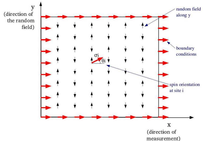
Figure 1: (color online) XY model on a 2D square lattice in a random magnetic field. The magnetic field is oriented along the y axis, \mathbf{h}_i = \eta_i \mathbf{e}_y , where \eta_i is a real random number. Right boundary conditions are assumed on the outer square, possibly placed at infinity (see text).
