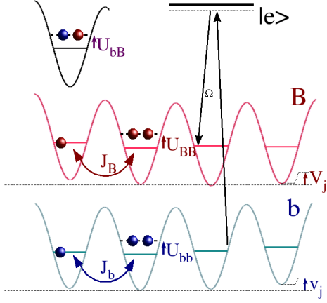
Figure 3: (color online) Atomic level scheme of a two-component Bose mixture in a random optical lattice used to design spin models in random magnetic fields (see text).
