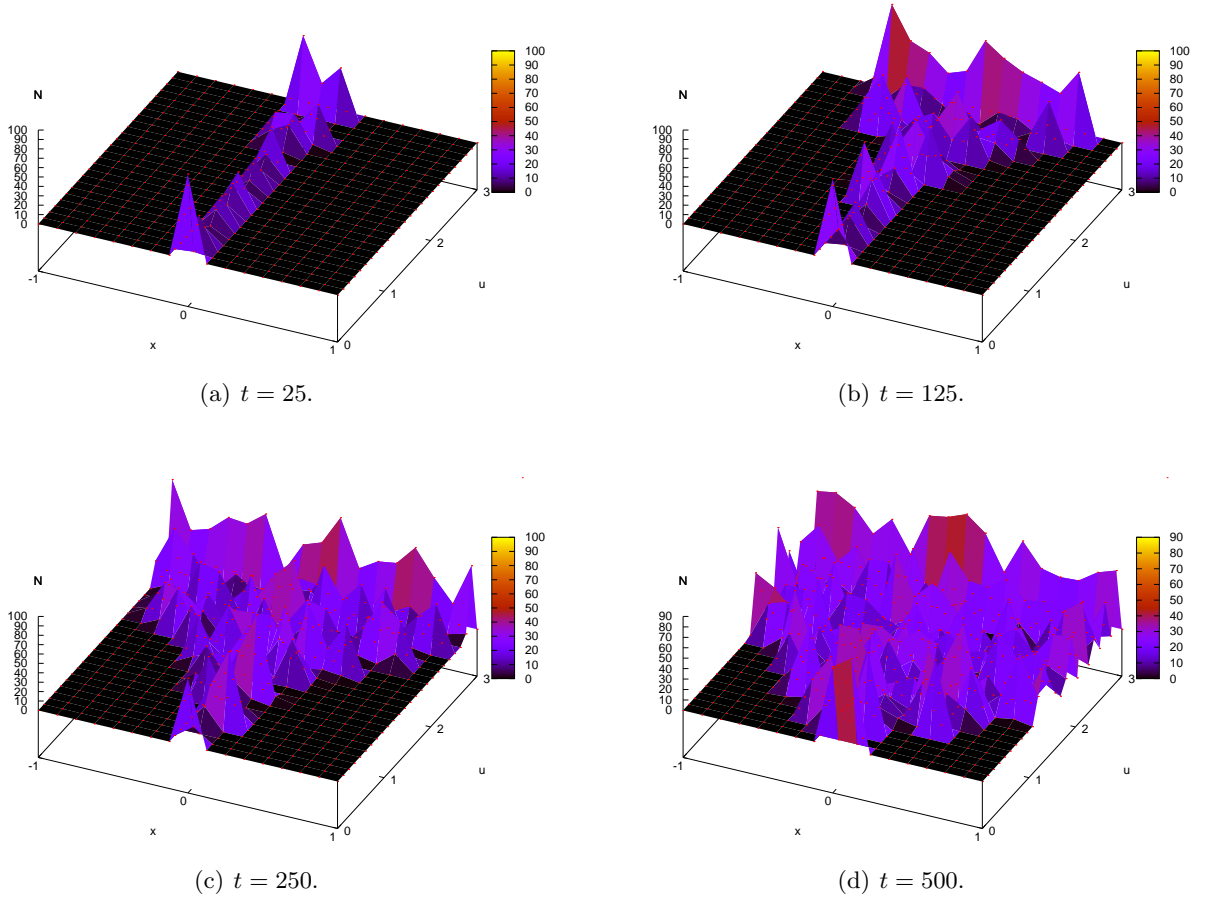
Figure 4: Simulations of Example 3. The parameters are N = 100, s = 0.03, m = 0.003 and \delta = 0.1 . The initial condition is composed of N individuals located at 0 and with trait values 3i/N for 1 \leq i \leq N .
