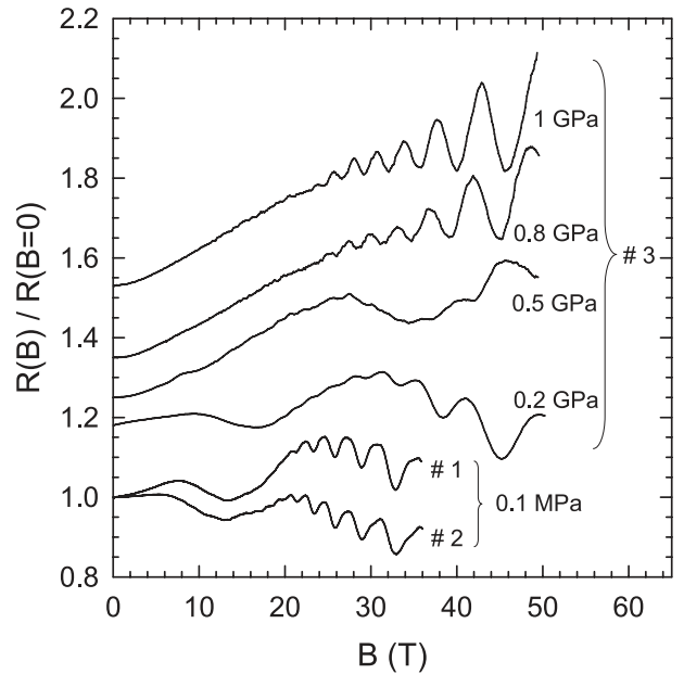
Fig. 3. Magnetoresistance at 2 K for various pressures (the low temperature values of which are given). The crystal number (see text) is indicated. Curves have been shifted from each other for clarity.
