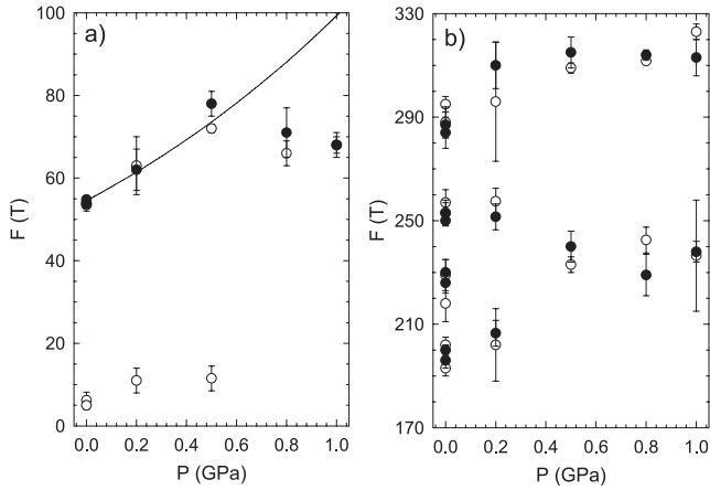
Fig. 9. Pressure dependence of the frequencies (a) F_0 and F_1 and (b) F_2 to F_5 , deduced from Fourier analysis (solid symbols) and fits of equation (6) (open symbols). The solid line is a fit of the equation F(P) = F(P=0)\exp(-\kappa P) , with \kappa = 0.6 \text{ GPa}^{-1} , to the data for F_1 .
