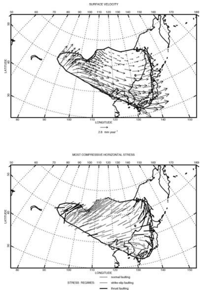
Figure 7. Same as Fig. 6 for model 2.
