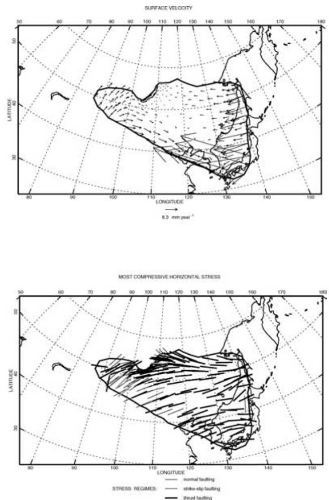
Figure 9. Same as Fig. 6 for model 7.
