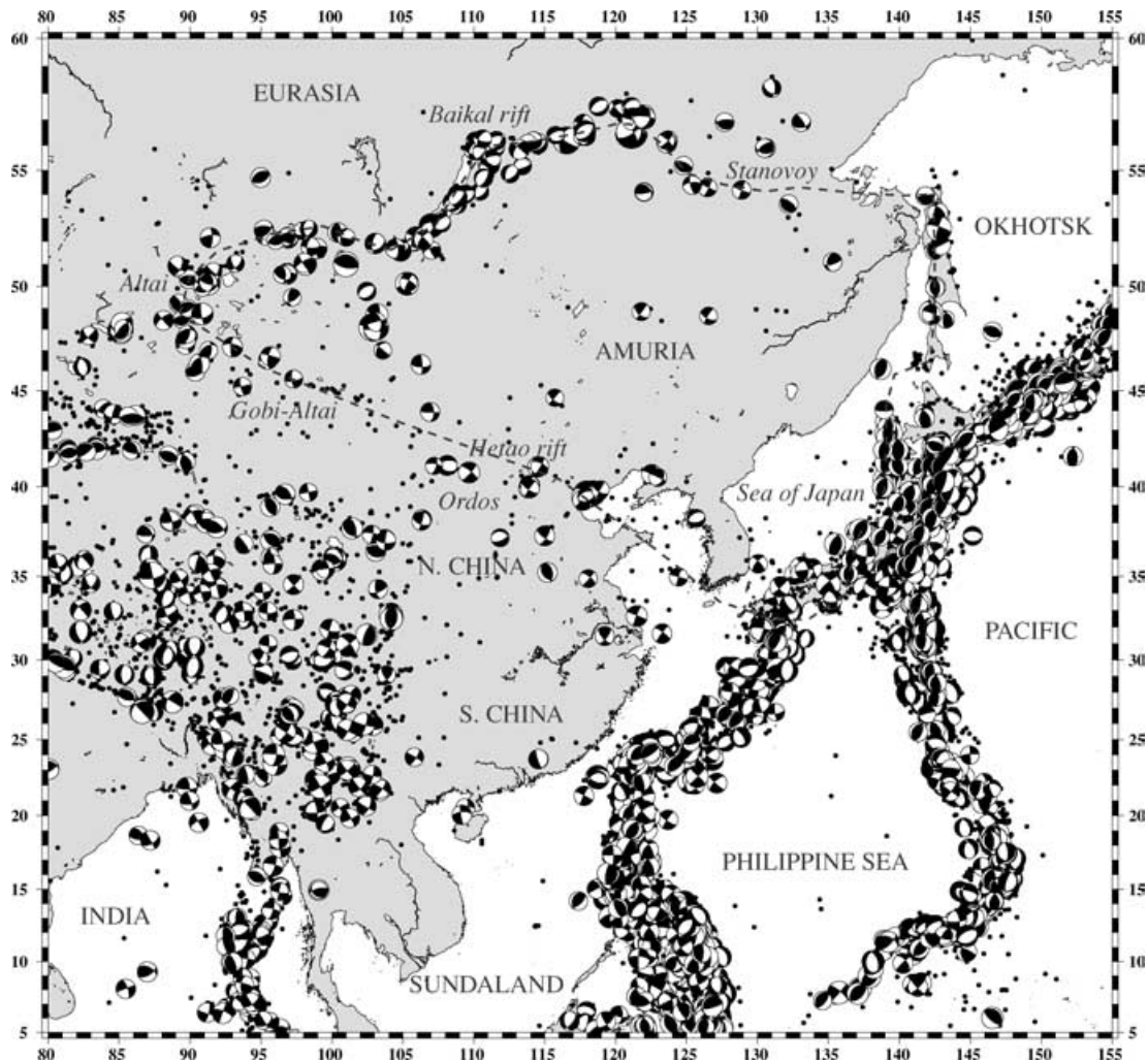
Figure 1. General setting and seismicity in eastern Asia. Epicentres come from the NEIC International Data Center (depth <50 km); focal solutions come from CMT (Dziewonski et al. 2003, and references therein) except for focal solutions and epicentres in the Stanovoy and Baikal regions which come from local data published in Parfenov et al. (1987) and Petit et al. (1996). The broken line indicates the inferred boundaries of the Amurian Plate.
